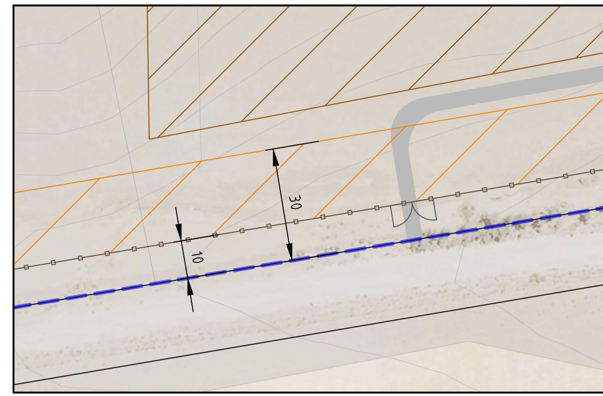
BOUNDARY OFFSETS (B) SCALE 1: 1000
